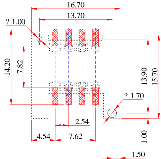
PCB
